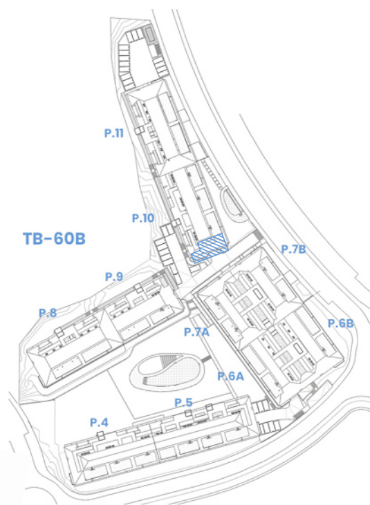
SITE PLAN
